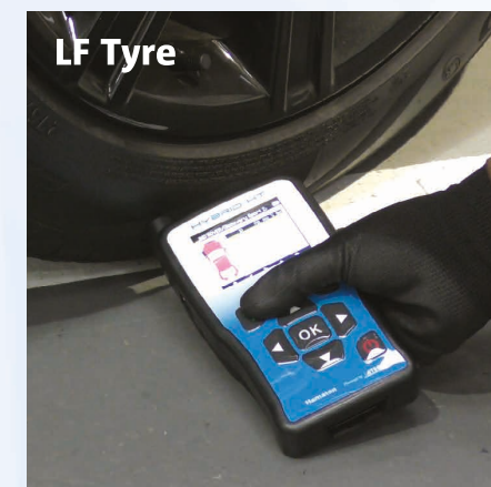
Place the tool on the sidewall near the valve, then press the green trigger button
