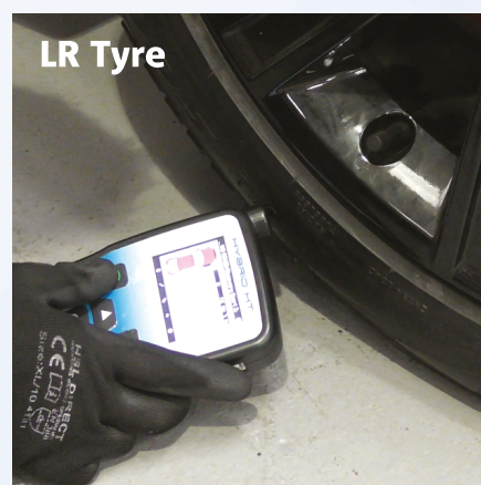
Repeat for the LR (left rear) tyre
