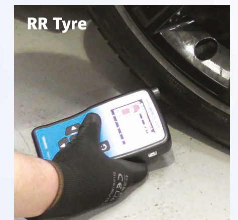
Repeat for the RR (right rear) tyre
